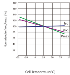
Power voltage current curve at different temperature
